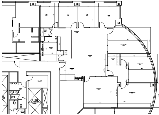
EXISTING FLOOR PLAN SCALE: Not to Scale
