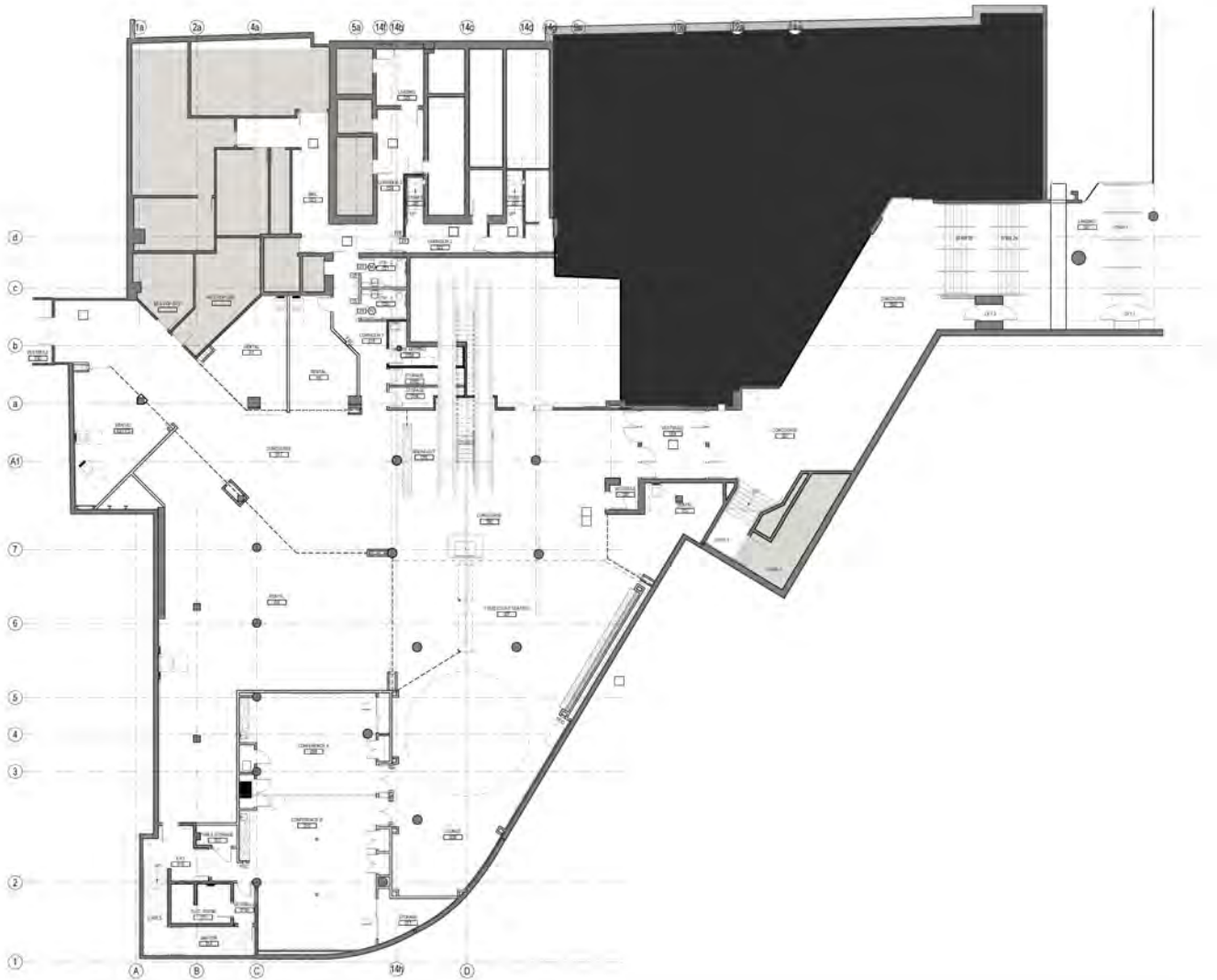
1 CONCOURSE - PLAN
